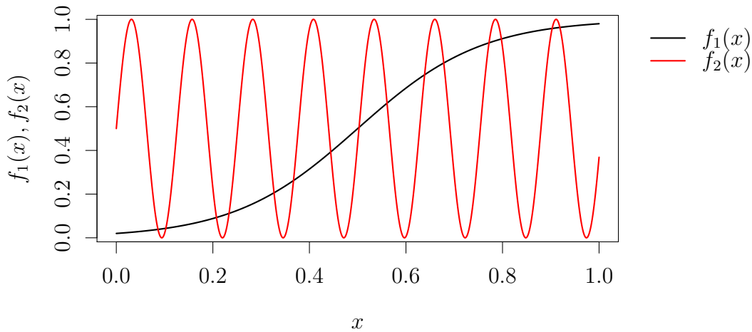
Figure 2.1: Plot of f_1 and f_2 of Equation (2.33).
