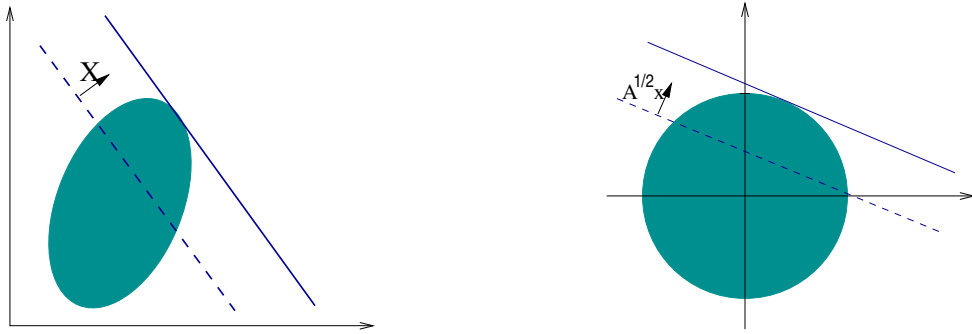
Figure 2.6: Reduction of linear optimization over an ellipsoid to linear optimization over a unit ball.
