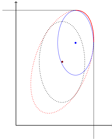
Figure 6.2: Approximating of the worst case subset (red) of the uncertainty set (red, dotted) through a more problem specific underestimator (blue).
