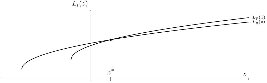
Figure 4.2: Label functions.
