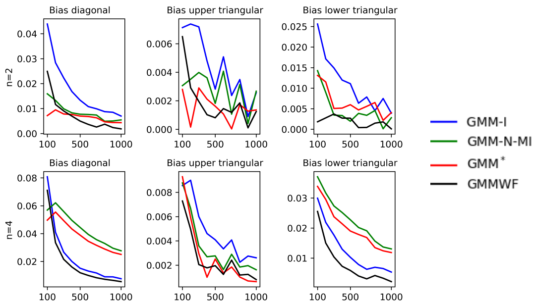
Figure 5: Average of the median absolute bias of the elements on the diagonal, upper- and lower-triangular of \hat{B} - One-step estimators
