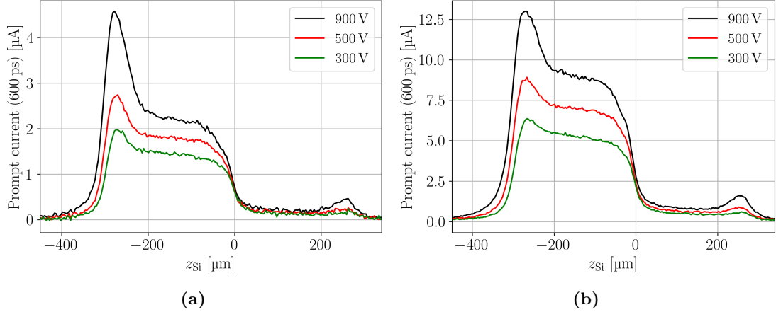
Figure 5.4: Prompt current profile of the W5-D8-LGAD2 LGAD for different bias voltages. The peak at z_{Si} \approx -280 \mu\text{m} corresponds to the multiplication layer at the top junction. The generated charge is 6.5 fC (a) and 27.5 fC (b).
