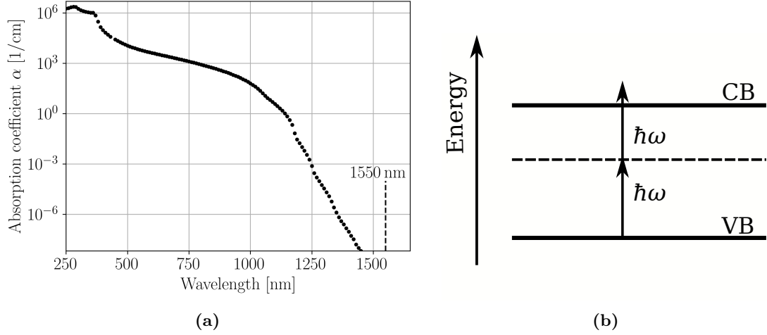
Figure 2.7: (a) Linear absorption coefficient of silicon at 300 K in intrinsic silicon. The data is taken from [81]. (b) Sketch of the excitation process via two photons in a semiconductor.
