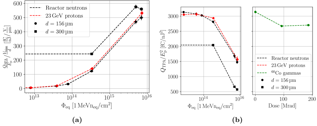
Figure 4.7: (a) SPA charge collection normalised with the average electric field versus the equivalent fluence for neutron and proton irradiated FZ p-type pad detectors from the CiS16 campaign. (b) TPA charge collection versus the equivalent fluence and dose for the same DUTs measured at a bias voltage of 300 V.
